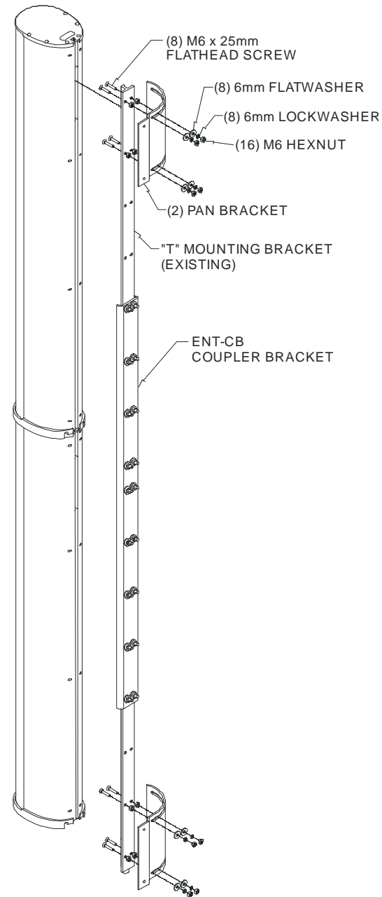
Figure 4: Pan Bracket Kit Assembly Diagram (Two Columns)
