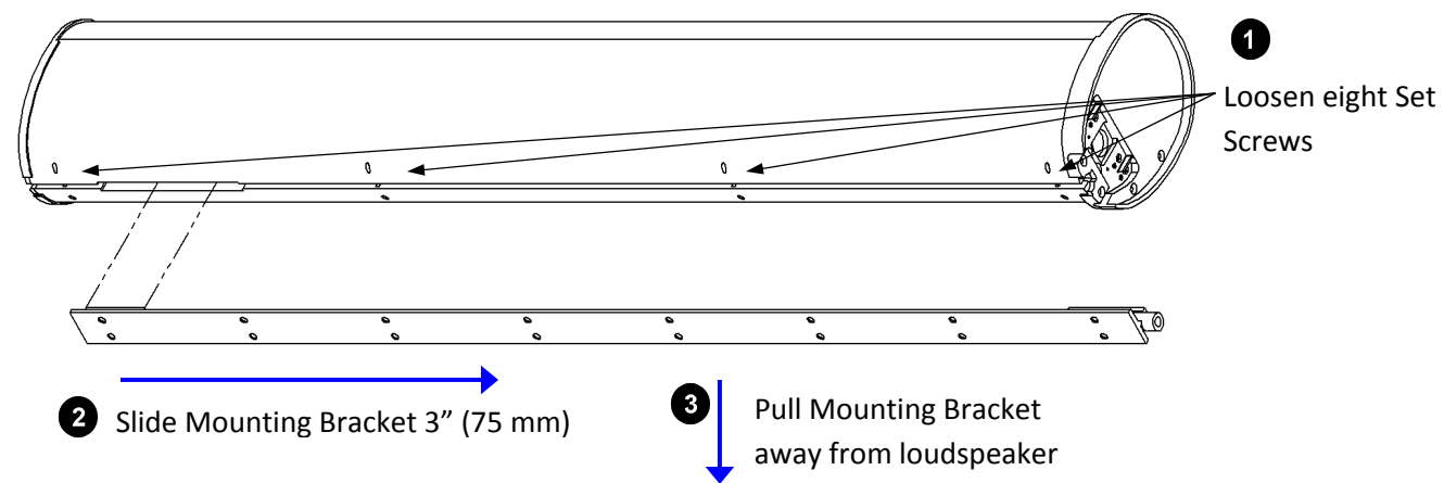
Figure 2: T-Bar Mounting Bracket Removal
