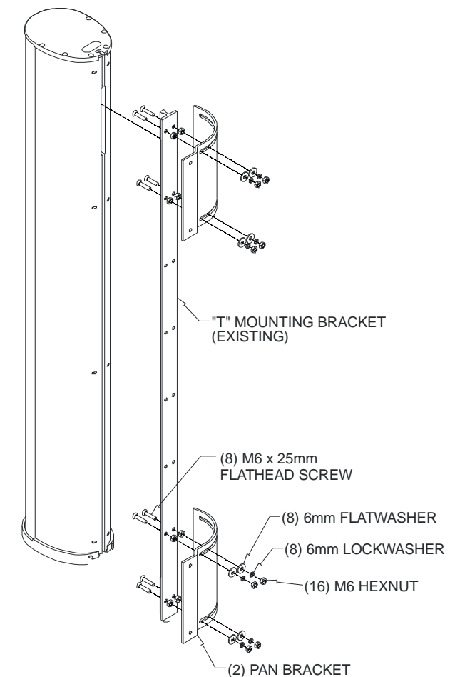
Figure 3: Pan Bracket Kit Assembly Diagram (One Column)
